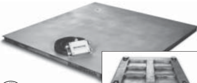
The 6" stainless steel channels provide superior protection for load cells and cable.
